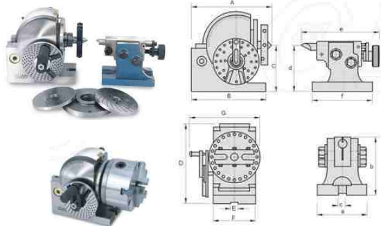
SEMI-UNIVERSAL INDEX CENTER B & S TYPE NO.0 , NO.1(HEAD-STOCK) Unit:mm
