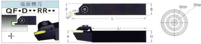
Radial cutting, the amount should not be too large Insert : Inquiry Parts : P01 Cutter diameter range
