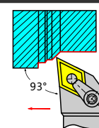
Main Angle 93°
