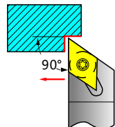
Main Angle 90°
