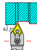
Main Angle 62.5°
