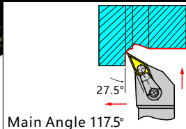
Main Angle 117.5°
