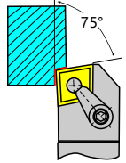
Main Angle 75°
