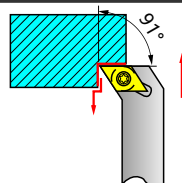
Main Angle 91°
